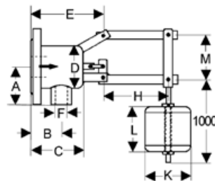
NV98 FPZ/u
