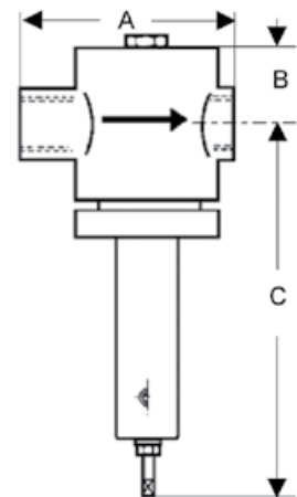
DM514 DM518
